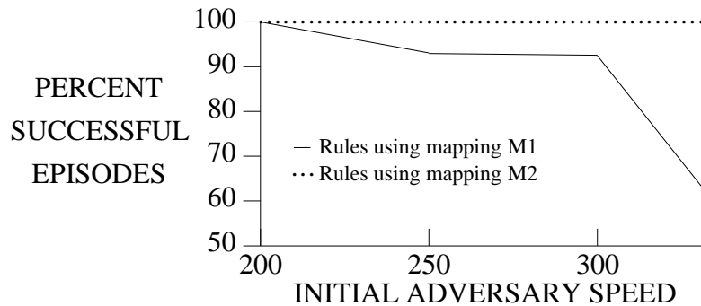
FIG. 2. Comparison of mappings on restricted EM.
