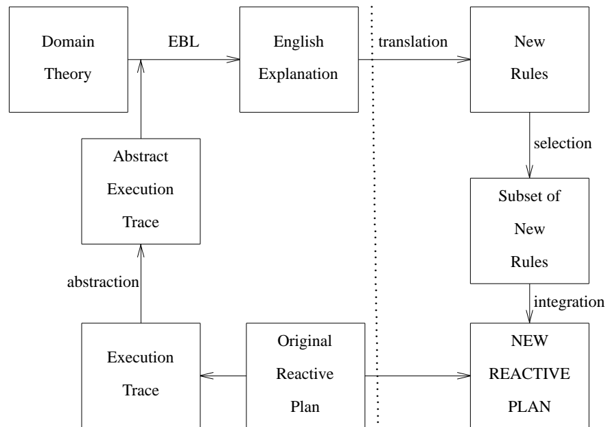
FIG. 1. Plan explanation and rule generation.
